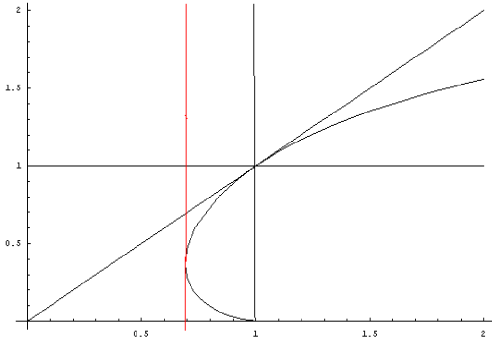
Plot of the square super-root (super square-root).
